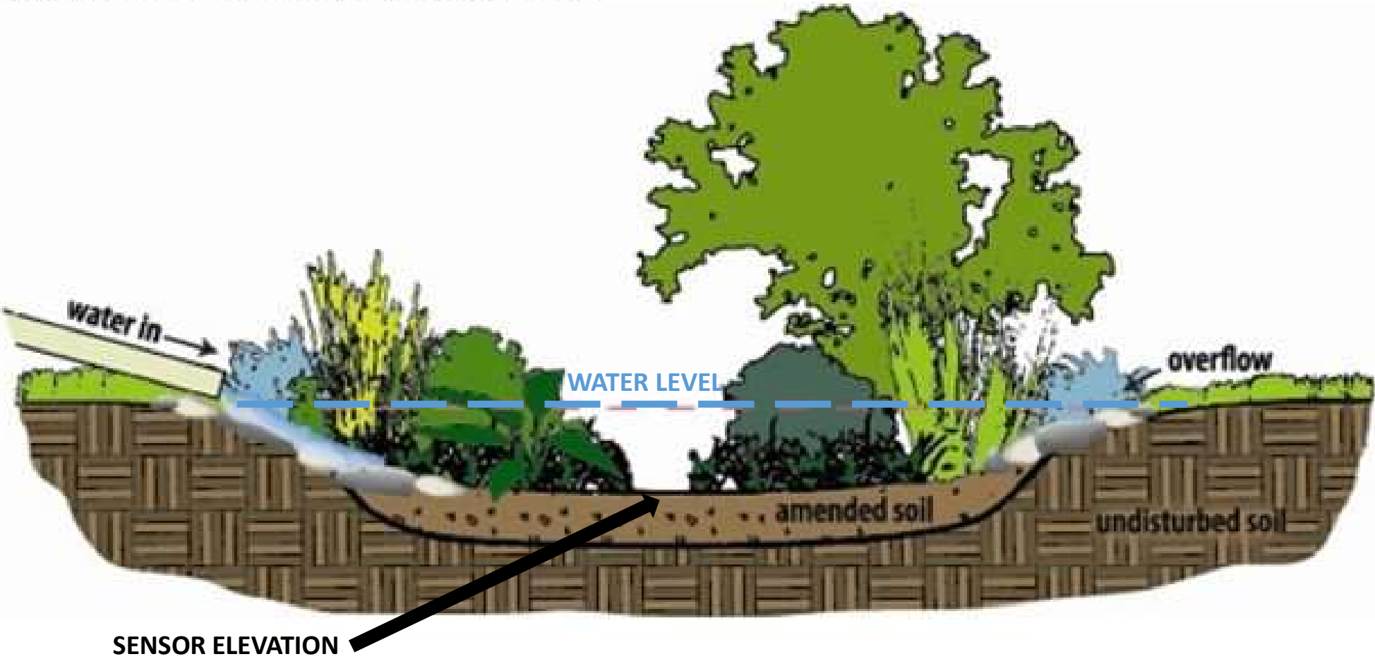
Caption: Cross-section of bio-infiltration BMP
